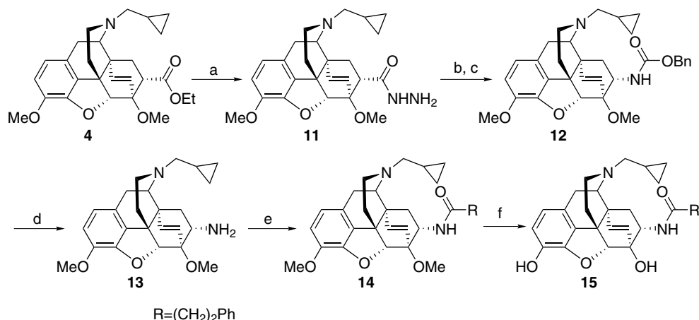
Scheme 5. Reagents and conditions: (a) \text{NH}_2\text{NH}_2 \cdot \text{H}_2\text{O} , 2-ethoxyethanol, reflux; (b) \text{NaNO}_2 aq, 6 M HCl; (c) BnOH, reflux, (d) AcOH, concd HCl, 80 °C; (e) \text{RCOCl} , \text{Et}_3\text{N} , \text{CH}_2\text{Cl}_2 , 0 °C; (f) \text{BBr}_3/\text{CH}_2\text{Cl}_2 , \text{CH}_2\text{Cl}_2 , rt.
