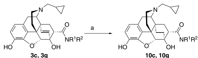
Scheme 4. Reagents and conditions: (a) \text{H}_2 , Pd/C, \text{CH}_3\text{SO}_3\text{H} , MeOH, rt.
