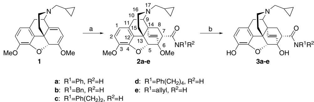
Scheme 1. Reagents and conditions: (a) N - R^1 - N - R^2 -acrylamide, xylene, reflux; (b) \text{BBr}_3/\text{CH}_2\text{Cl}_2 , \text{CH}_2\text{Cl}_2 , rt. Numbering of atoms in 6,14-endo-ethenomorphinan is shown in formula 2 .
