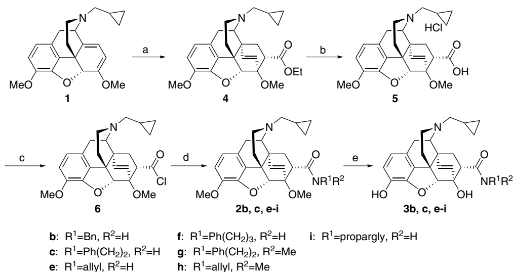
Scheme 2. Reagents and conditions: (a) ethyl acrylate, reflux; (b) 6 M \text{HCl} , reflux; (c) (\text{COCl})_2 , \text{CHCl}_3 , reflux; (d) \text{HNR}^1\text{R}^2 , \text{Et}_3\text{N} , \text{CH}_2\text{Cl}_2 , 0^\circ\text{C} ; (e) \text{BBr}_3/\text{CH}_2\text{Cl}_2 , \text{CH}_2\text{Cl}_2 , rt.
