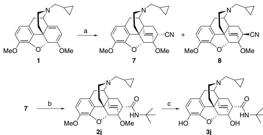
Scheme 3. Reagents and conditions: (a) acrylonitrile, reflux; (b) t - \text{BuOH} , 85% \text{H}_2\text{SO}_4 , \text{AcOH} , rt; (c) \text{BBr}_3/\text{CH}_2\text{Cl}_2 , \text{CH}_2\text{Cl}_2 , rt.
